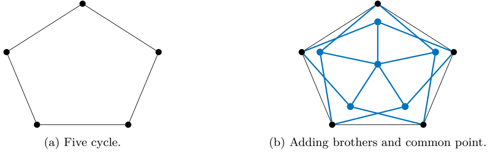
Figure 5.1: Mycielski creation of a graph.
